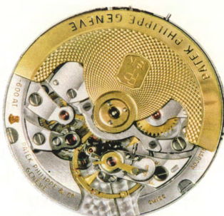
12-600 AT Movement Ø: 27.07 mm (1953)
