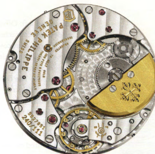
240 Movement Ø: 27.5 mm (1977)
